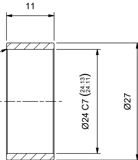
SECTION A-A (2:1)
